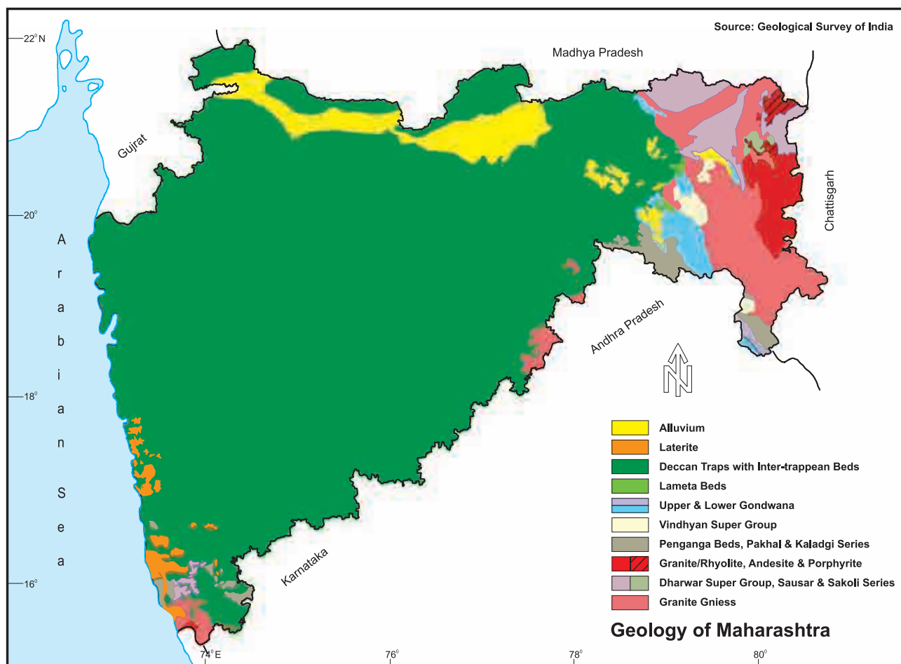
Fig. 6.2 : The generalized Geological map of Maharashtra
